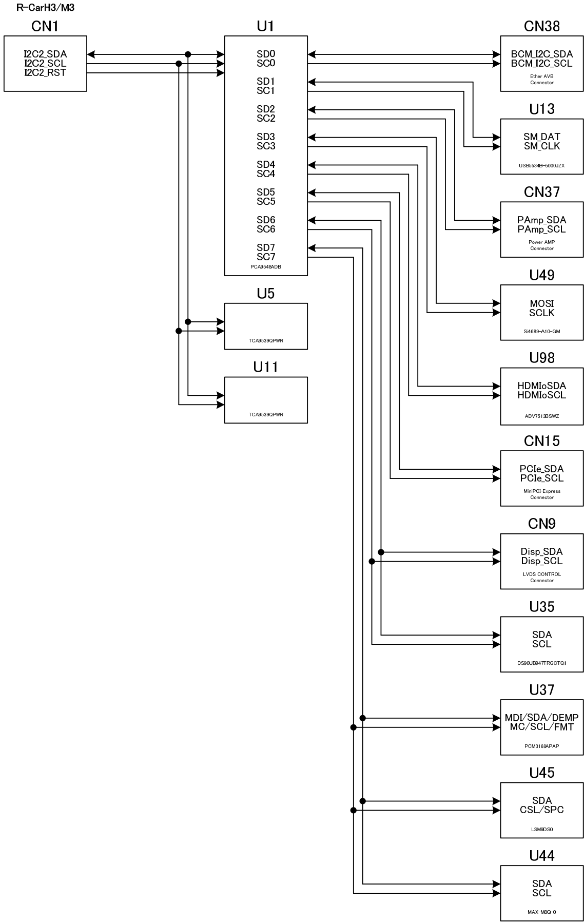
Figure 4-23a : I2C I/F
