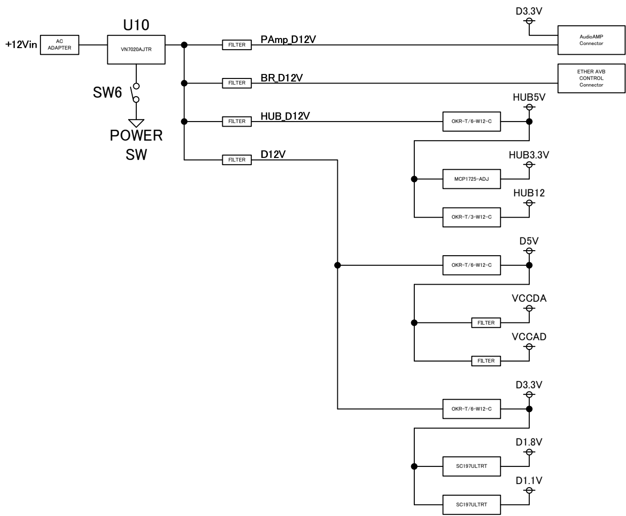
Figure 4-1 : Power structure
