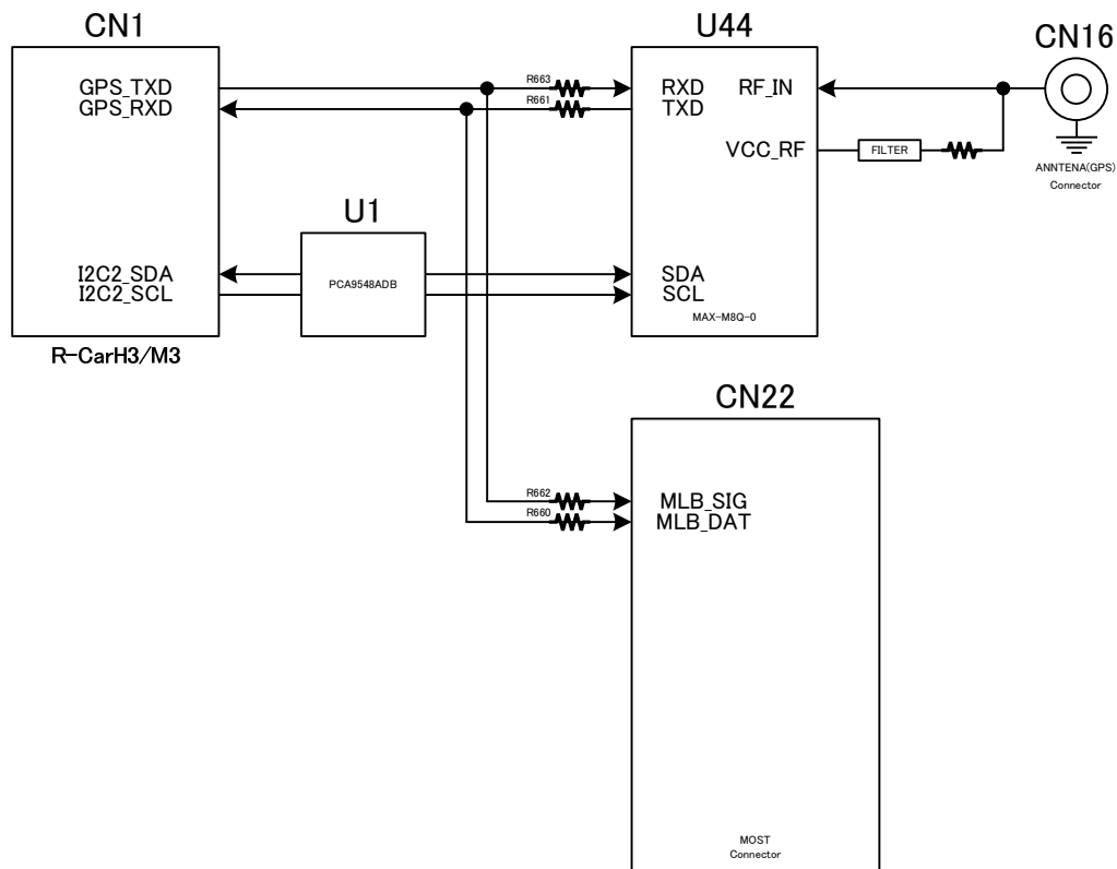
Figure 4-19: GPS I/F
