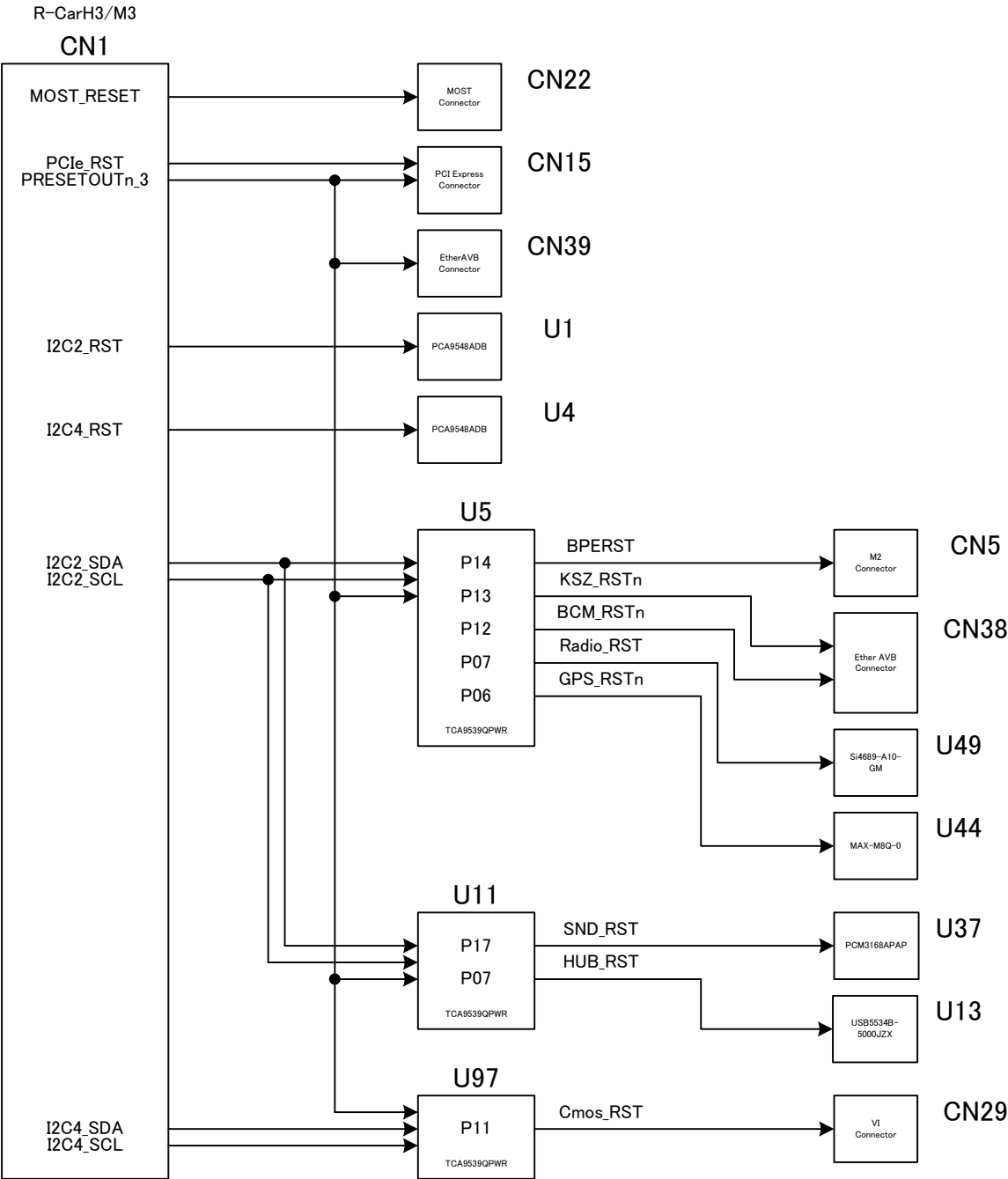
Figure 4-2 : Reset structure
