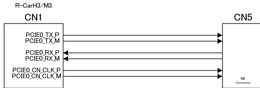
Figure 4-7: M2 I/F
