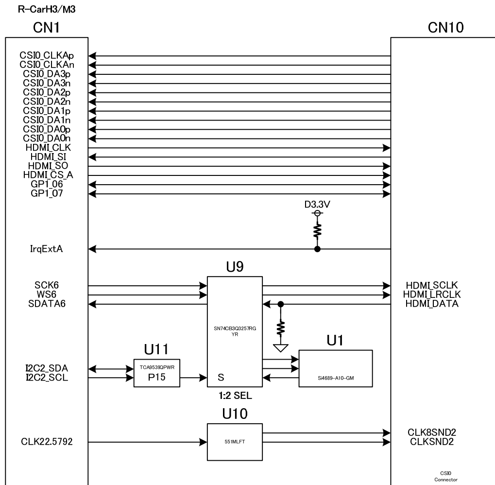
Figure 4-11a : camera SERIAL interface (CSI0) I/F
